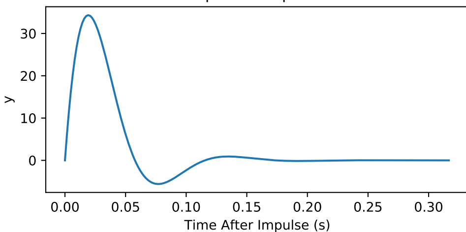
Impulse-Response
