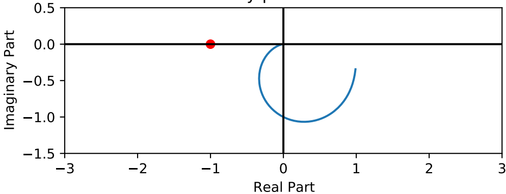
Nyquist Plot
