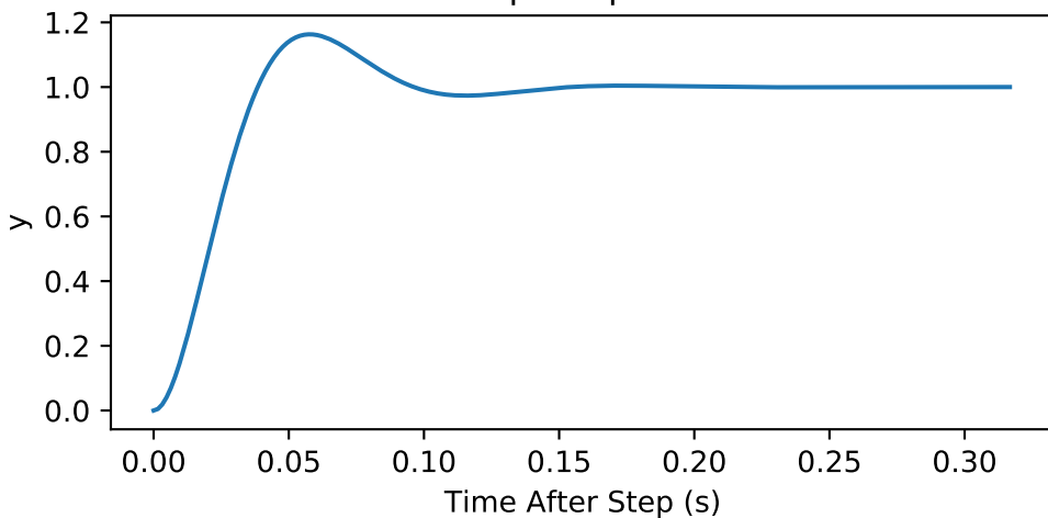
Step-Response
