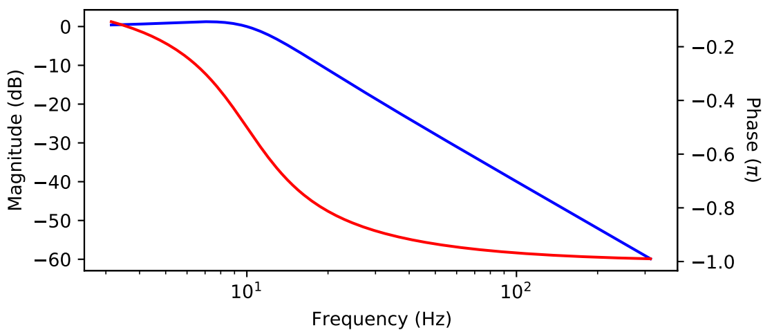
Bode Plot
